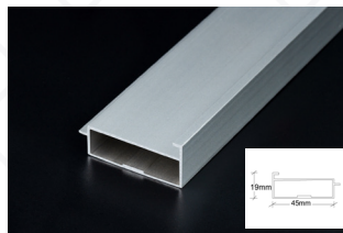
3G FRAME
